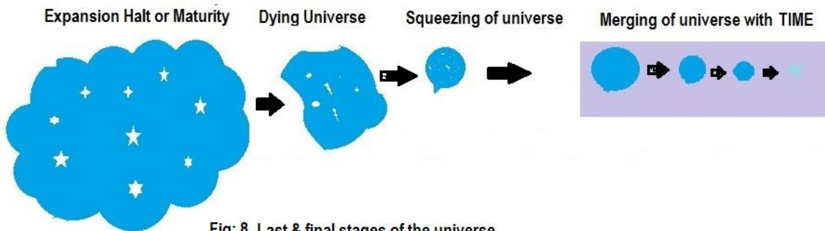
Fig: 8 Last & final stages of the universe
