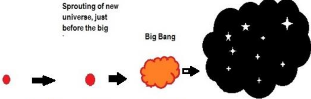
Fig: 6 Stages of universe before big bang
