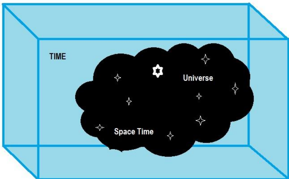
Fig: 4 Shows TIME & Space Time.
