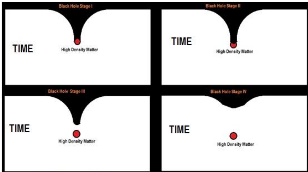
Fig 7: Stages of Black hole
